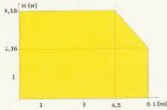
Up and Over door
