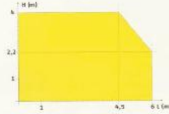
Sectional door
