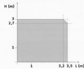
Sectional door
